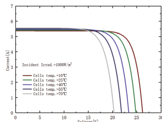
I-V Curves of 100W at different cell temperature
