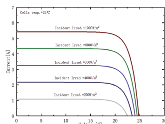
I-V Curves of 100W at different irradiance
